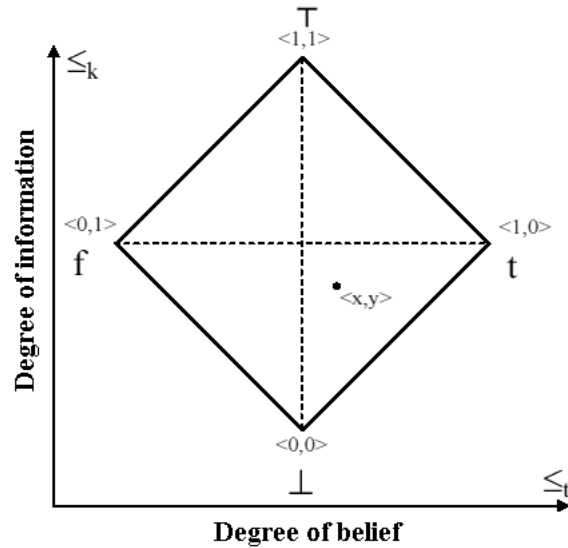
Figure 4 The bilattice square \mathcal{B} = ([0, 1]^2, \leq_t, \leq_k) . Every element of this bilattice is of the form \langle \text{evidence\_for}, \text{evidence\_against} \rangle .
