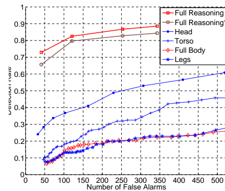
Figure 10 ROC curves for evaluation on Dataset-A. Full Reasoning* is ROC curve for 126 occluded humans.
