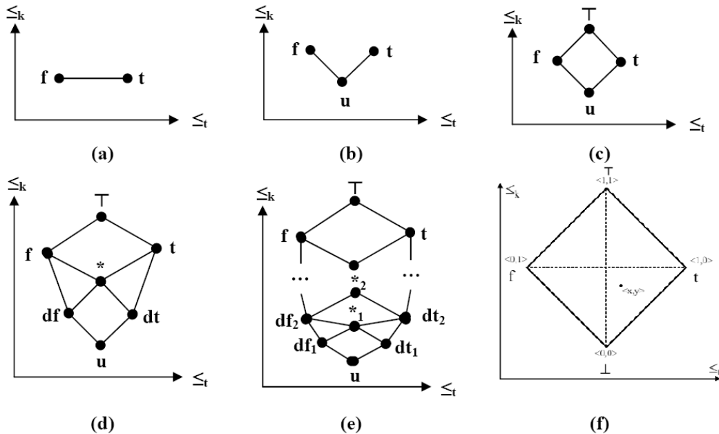
Figure 3 The choice of different lattices that compose the bilattice give rise to different logics. (a) bilattice for two valued logics (trivial bilattice) with only true and false nodes (b) bilattice for three valued logic with additional node for unknown (c) bilattice for four valued logics with additional node for contradiction (d) bilattice for default logics [17,39] where dt, df and * represent true by default, false by default and contradiction between dt-df respectively (e) bilattice for prioritized default logics [17,39] with different levels of defaults and (e) bilattice for continuous valued logic [3,40] as described in this paper.
