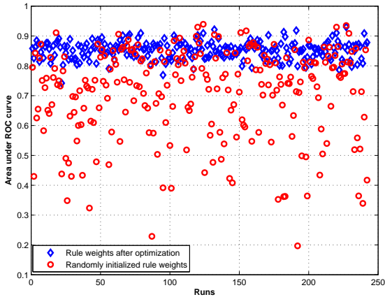
Figure 14 Plot showing area under ROC curve for random initialization of rule weights and trained rules for multiple runs on the USC_CAVIAR dataset.
