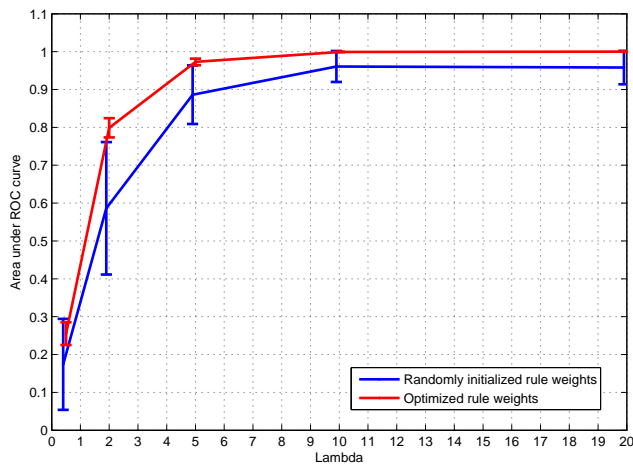
Figure 16 Plot showing mean AUROC and associated variance on simulated data for varying values of \lambda
