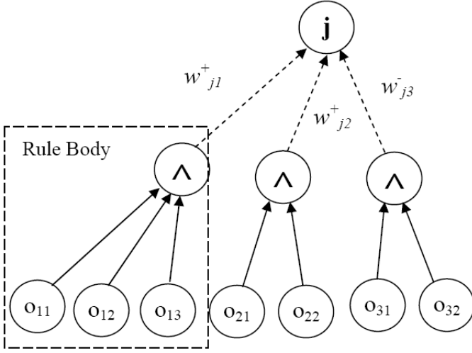
Figure 13 Example of a knowledge based artificial neural network representing rules depicted in (5).
