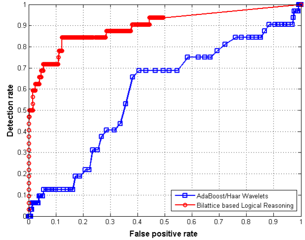
Figure 11 ROC Curves for SAM site detection problem.
