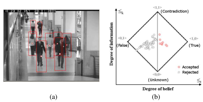
Figure 7 (a) Figure showing a sample image from the USC_CAVIAR dataset with detection results overlaid and (b) Computed uncertainty value (for all human hypotheses in left image) plotted in the bilattice space.
